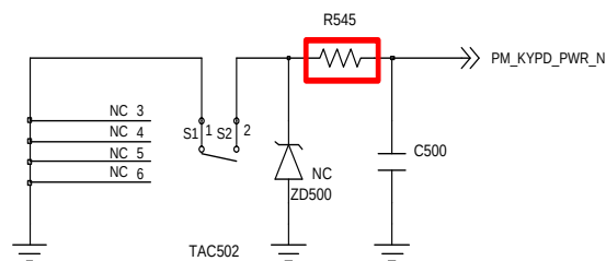
Power-ON / Hold Key
